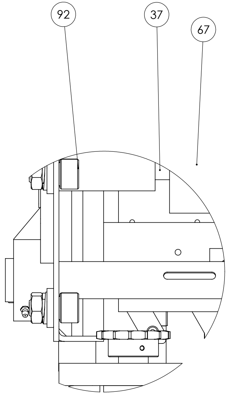
DETAIL B SCALE 1:2
